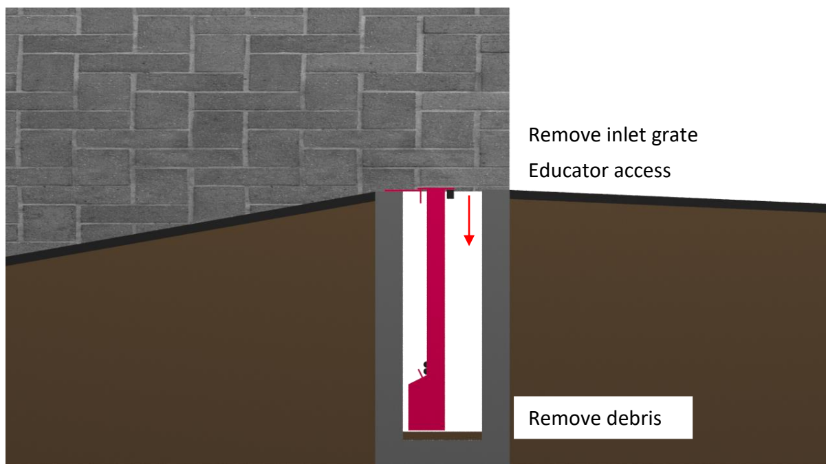
Figure 10 - FD Flood Barrier Maintenance
